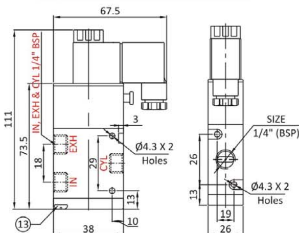
Size : 1/4" BSP (Dimensions are in mm)
