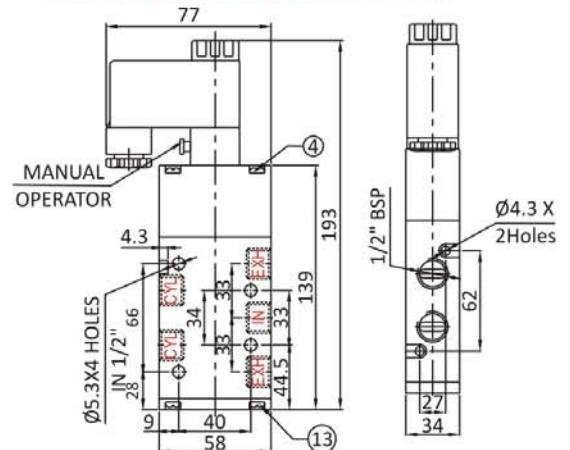
Size : 1/2" BSP (Dimensions are in mm)
