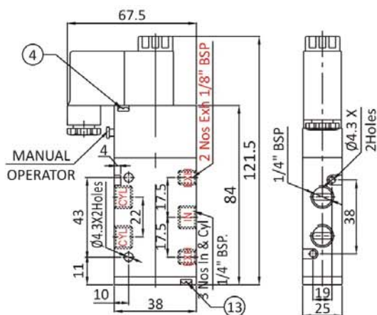
Size : 1/4" BSP (Dimensions are in mm)
